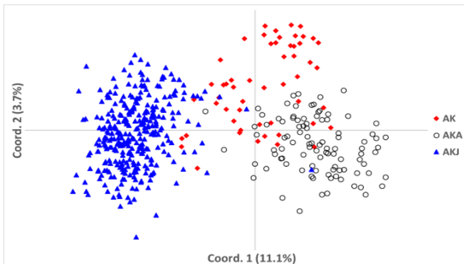
Fig. 1. Top- PCoA of 524 Akitas from three different populations – Akita blend (AK), American Akita (AKA), and Japanese Akita (AKJ)
