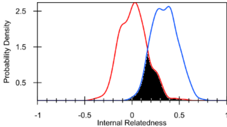
Fig. 3: Distribution of IR estimates in 341 AKJ based on intra-breed diversity (Red line), compared with IR adjusted for diversity lost during breed development (Blue line). Diversity lost because of breed development was determined by comparing allele frequencies at the same loci between AKA and randomly breeding village dogs from the Middle East, SE Asia, and the Pacific Islands. The area in black is an estimate of how much available genetic diversity has been retained (24.4%) or lost (75.6%) during the evolution of contemporary AKJ.
