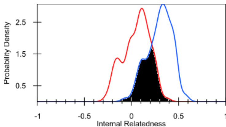
Fig. 2: Distribution of IR estimates in 117 AKA based on intra-breed diversity (Red line), compared with IR adjusted for diversity lost during breed development (Blue line). An estimate of diversity lost because of breed development (area in black) was determined by comparing allele frequencies at the same loci between AKA and randomly breeding village dogs from the Middle East, SE Asia, and the Pacific Islands. The area in black is an estimate of how much available genetic diversity has been retained (41%) or lost (59%) in during the evolution of contemporary AKJ. Retention of 41% village dog diversity is above average for pure breeds.
