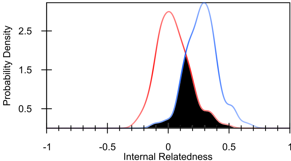
Fig. 3. Distribution of IR estimated in Samoyed (n=190) based on intra-breed diversity (red line), compared with IR adjusted for available genetic diversity that has been lost during breed development (blue line). The black area is an estimate of lost genetic diversity using randomly breeding village dogs as the standard.
